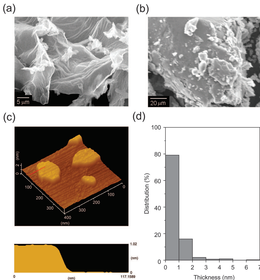
Figure 2. SEM images of (a) freeze-dried aggregate of MnO 2 monosheets and (b) self-assembled K/MnO 2 . (c) Tapping-mode AFM image of MnO 2 monosheets and height profile along the red line in the image. The monosheets are deposited onto fluorinated mica substrate precoated with poly(ethyleneimine) by spin-coating (1000 rpm for 15 s and 2000 rpm for 30 s) of 0.1 g L -1 colloidal suspension. (d) Histogram of thickness of the MnO 2 sheets on the substrate.
