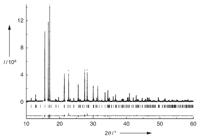
Figure 3. Structural characterization of \text{Sr}_3\text{Fe}_2\text{O}_5 by Rietveld refinement of synchrotron XRD data at 293 K. The overlying crosses, solid lines, and ticks represent the observed and calculated intensities and the position of the calculated Bragg reflections, respectively. The difference between the calculated and observed profiles is plotted at the bottom. \text{Sr}_3\text{Fe}_2\text{O}_5 adopts the Immm space group (No. 71), a=3.514825(2) , b=3.95271(2) , c=20.91252(10) Å, Z=2 . Sr(1) on 2c (0.5,0.5,0), Sr(2) on 4i (0,0,0.31234(2)), Fe on 4i (0,0,0.09636(2)), O(1) on 2a (0,0,0), O(2) on 4j (0.5,0,0.59574), O(3) on 4i (0,0,0.19358(2)), with 100% occupancy, B_{\text{iso}}(\text{Sr}(1))=0.359(22) Å 2 , B_{\text{iso}}(\text{Sr}(2))=0.213(13) Å 2 , B_{\text{iso}}(\text{Fe})=0.089(16) Å 2 , B_{\text{iso}}(\text{O}(1))=0.12(11) Å 2 , B_{\text{iso}}(\text{O}(2))=0.15(6) Å 2 , B_{\text{iso}}(\text{O}(3))=0.59(8) Å 2 , R_p=0.0401 , R_{\text{wp}}=0.0524 , and \chi^2=5.28 . Refining the occupation factors at the oxygen sites and the vacant site did not improve the result.
